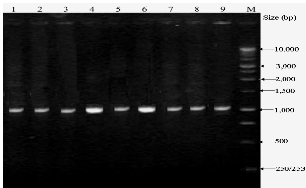
Fig. 4: Agarose gel photograph showing acdS gene fragment (1.0 kb) in nine selected isolates. Lane 1 to 9: acdS gene fragment of various strains ( Klebsiella sp strain ECI-10A, Microbacterium sp strain ECI-12A, Agrobacterium sp strain AF-1D, Pseudomonas sp strain AF-4B, Serratia sp strain AF-5A, Klebsiella sp strain AF-4C, Pseudomonas sp strain PN-4D, Agrobacterium sp strain BN-2A, and Klebsiella sp strain BN-4A); M: 1.0 kb DNA marker.
